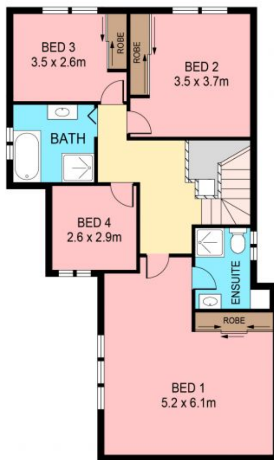
LEVEL ONE
